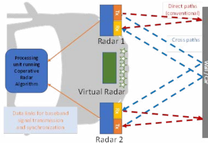
Figure 10: Secondary radar principle of operation and resulting virtual radar.
