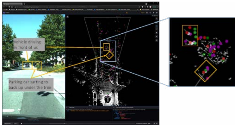
Figure 11: Enhanced point cloud in test drives: Ground truth data and camera data shown, radar reflections from left radar in red, right radar in green and virtual radar in magenta.
